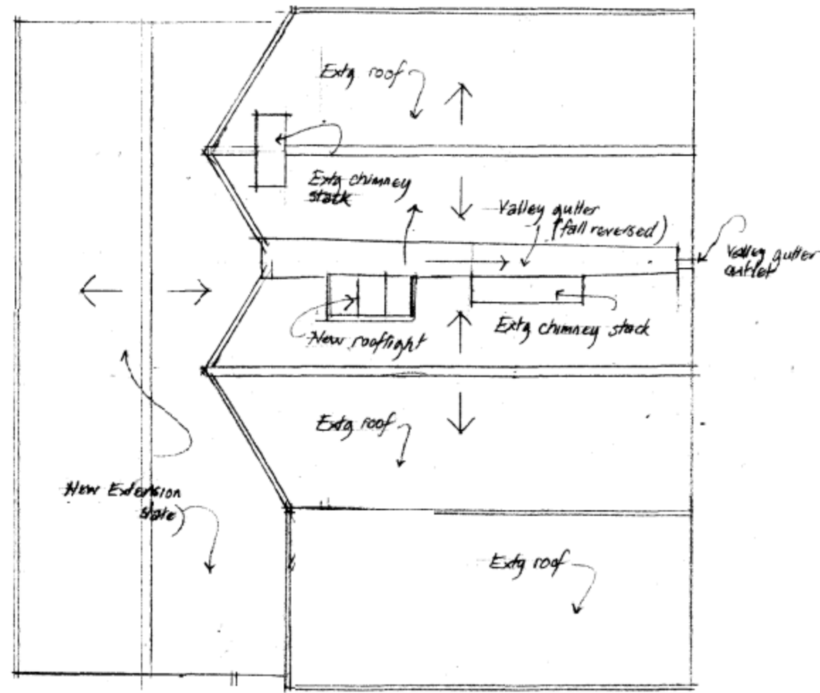
Roof Plan
