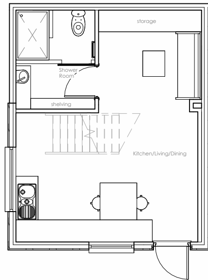
2 Ground Floor Plan - Proposed 1 : 100
