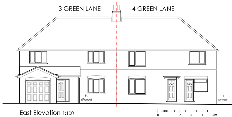
East Elevation 1:100
