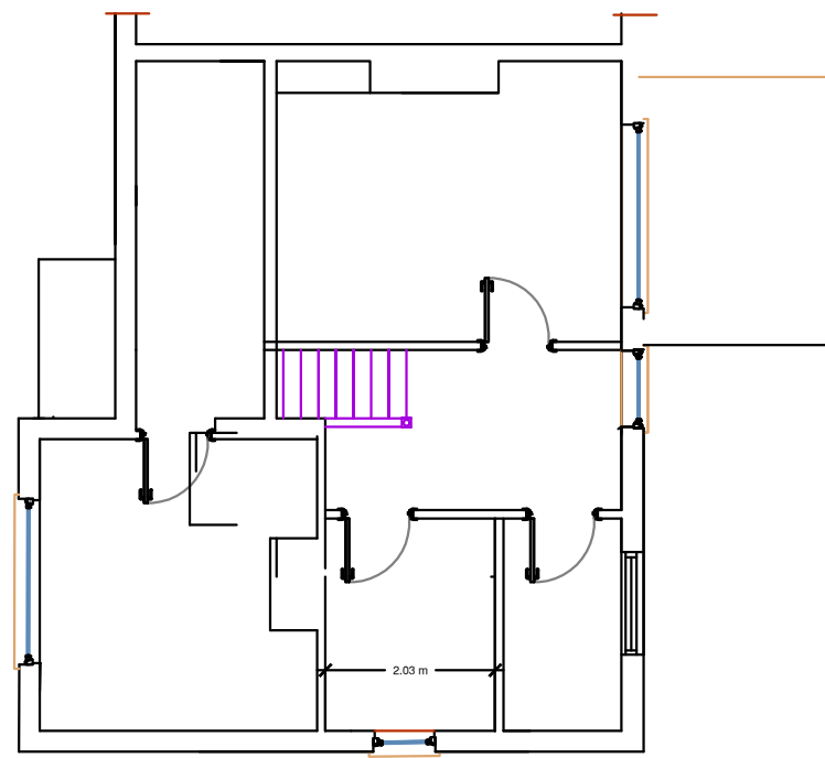
FIRST FLOOR PLAN AS EXISTING
