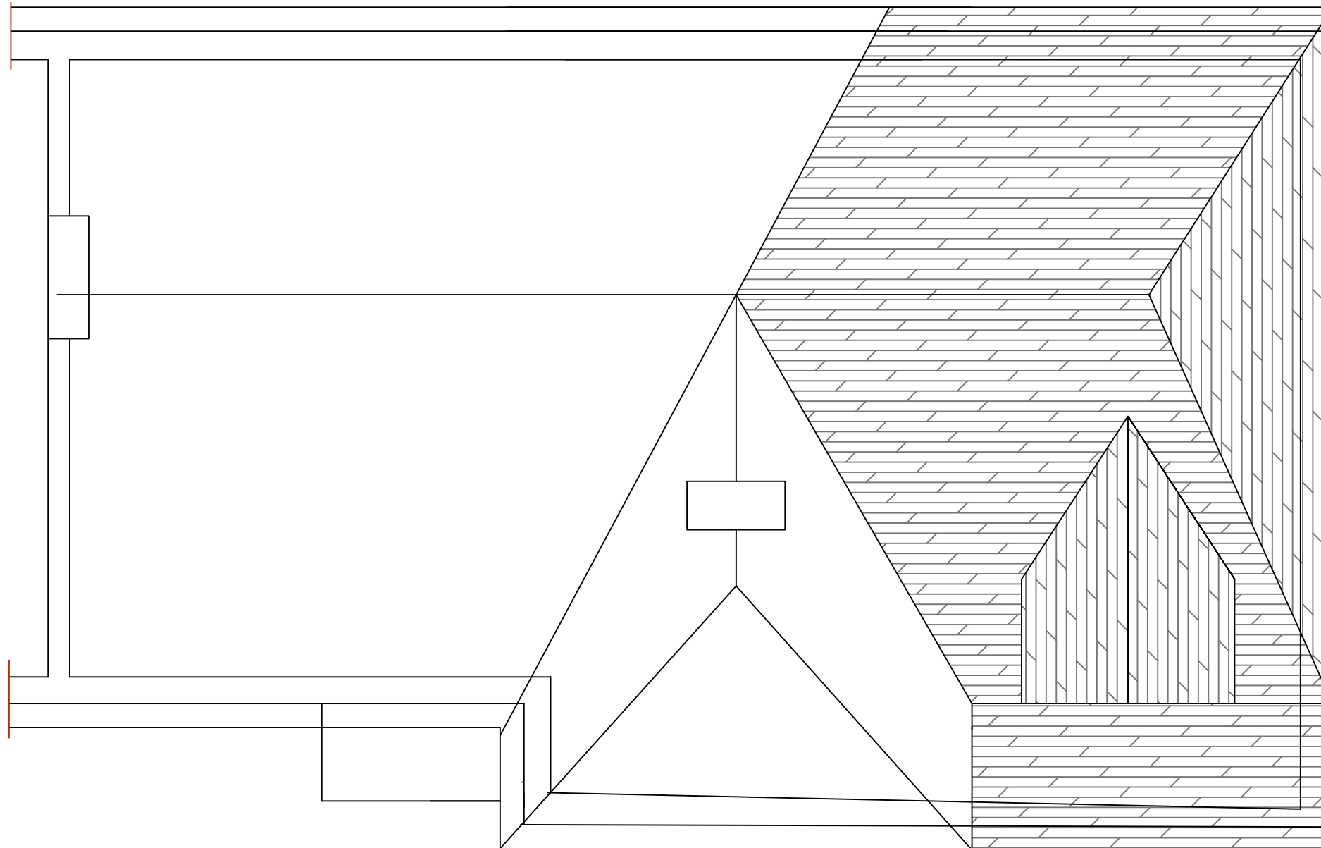
ROOF PLAN AS PROPOSED
