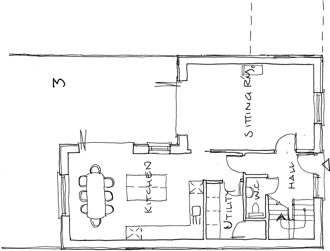
GROUND FLOOR ~ PLOT 3 1:100
