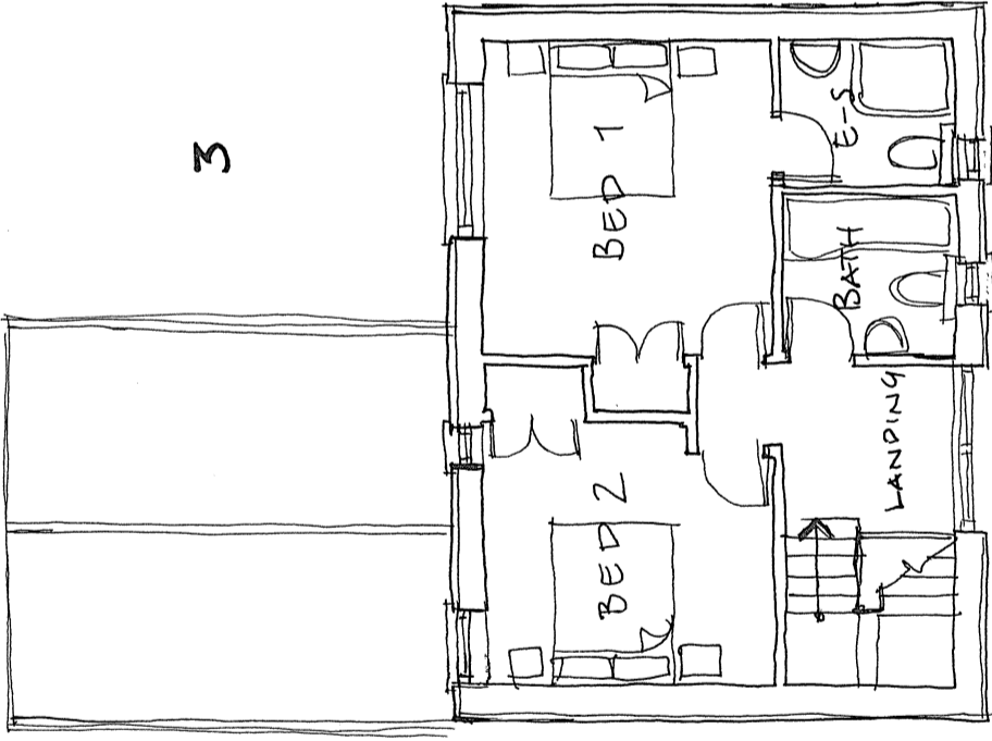
FIRST FLOOR PLOTS 3 1:100
