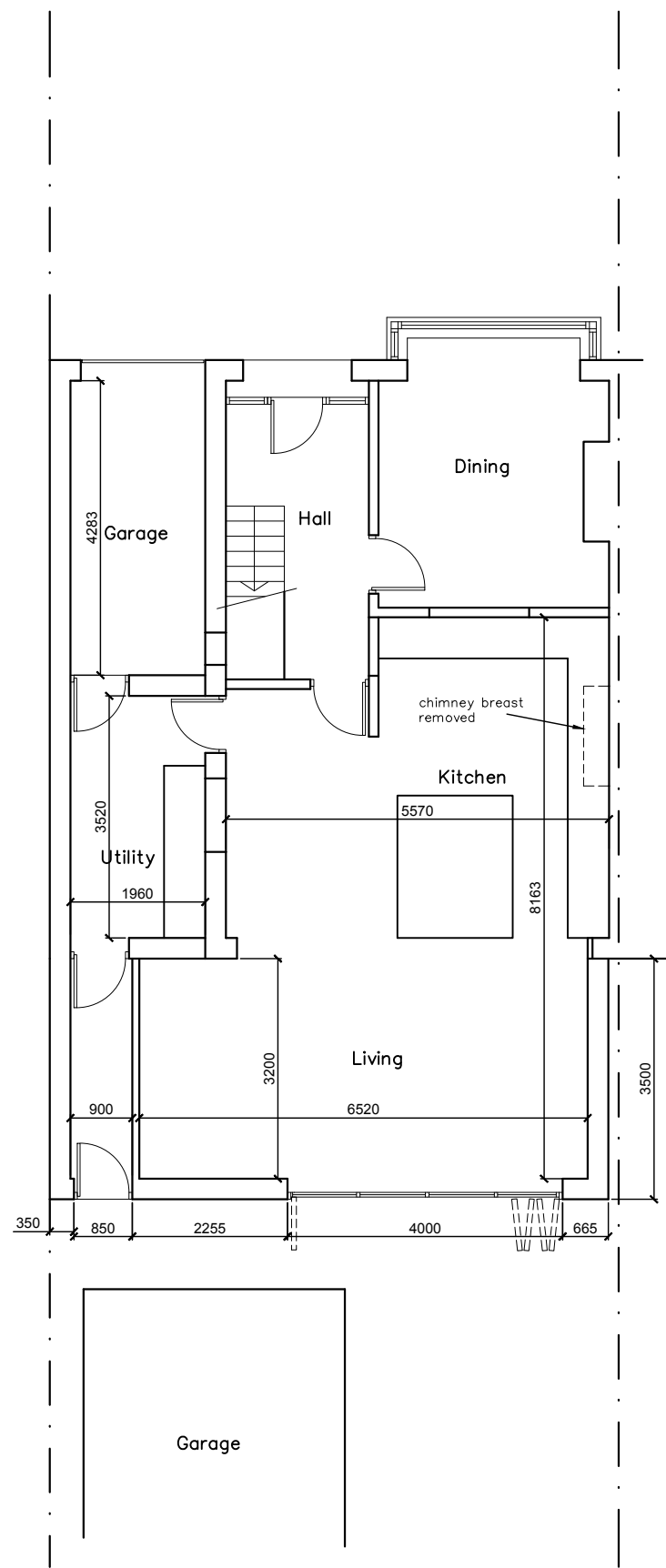
GROUND FLOOR
