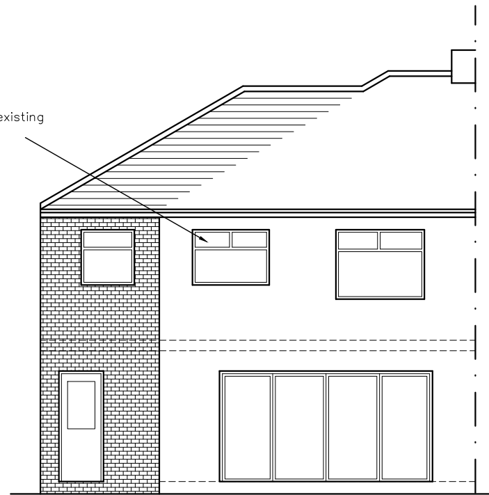
REAR ELEVATION
