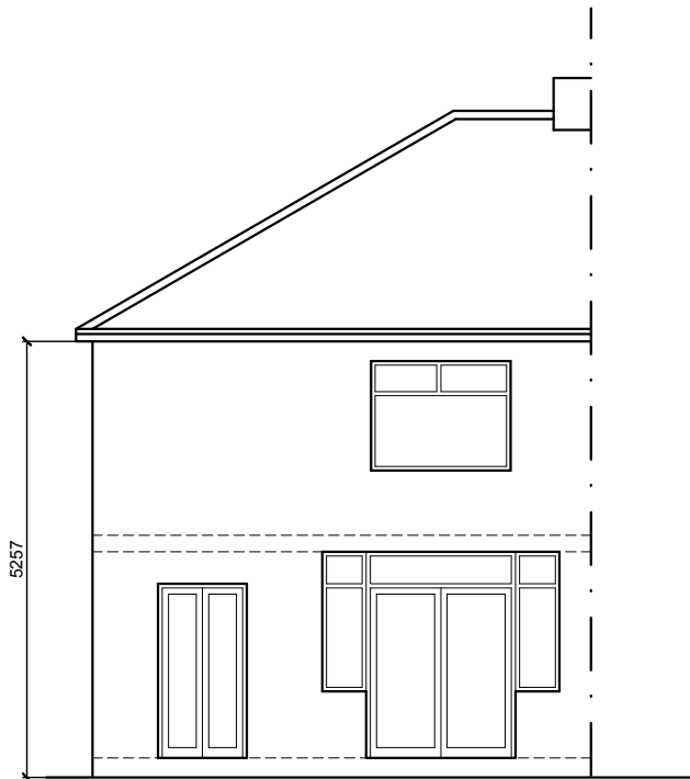
REAR ELEVATION
