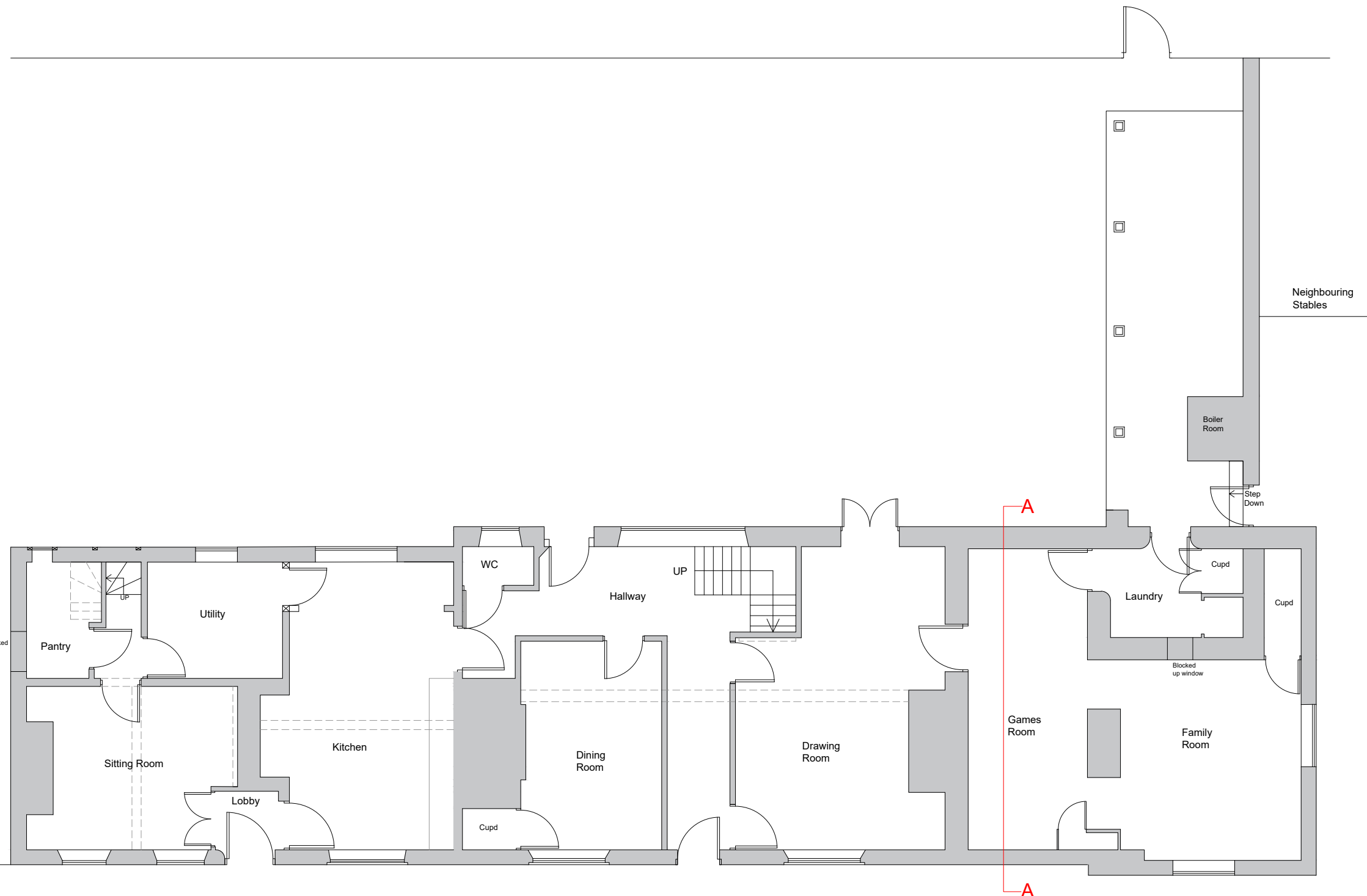
Existing Ground Floor Plan 1:100
