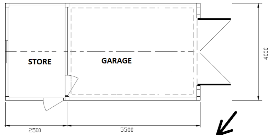
PLAN & ROOF PLAN
