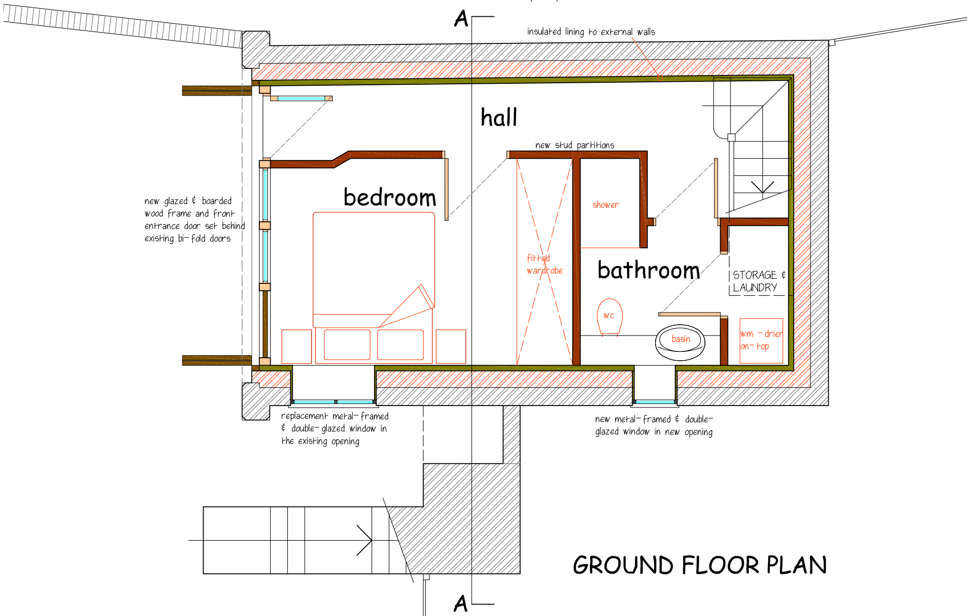
FLOOR LAYOUT PLANS conversion to dwelling annex
