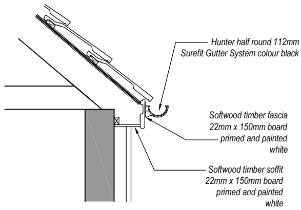
Soffit/Eaves Detail Scale 1:20
