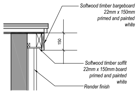
Verge Detail Scale 1:20
