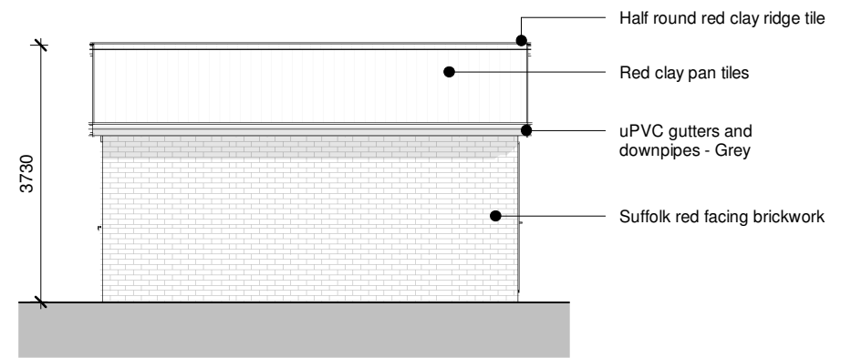
South Elevation As Proposed 1 : 100
