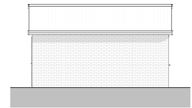
North Elevation As Proposed 1 : 100
