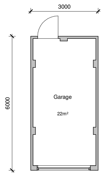
GA Ground Floor Plan As Proposed 1 : 100
