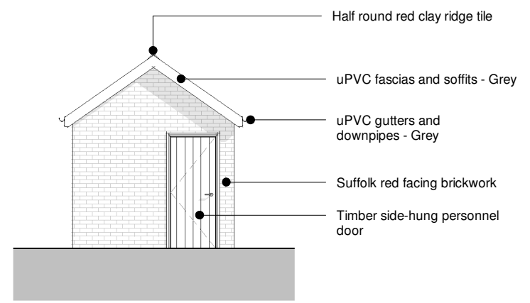
West Elevation As Proposed 1 : 100
