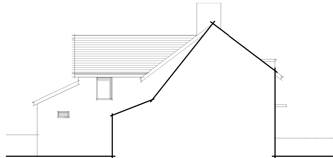
Existing Side / East Elevation 1 : 100
