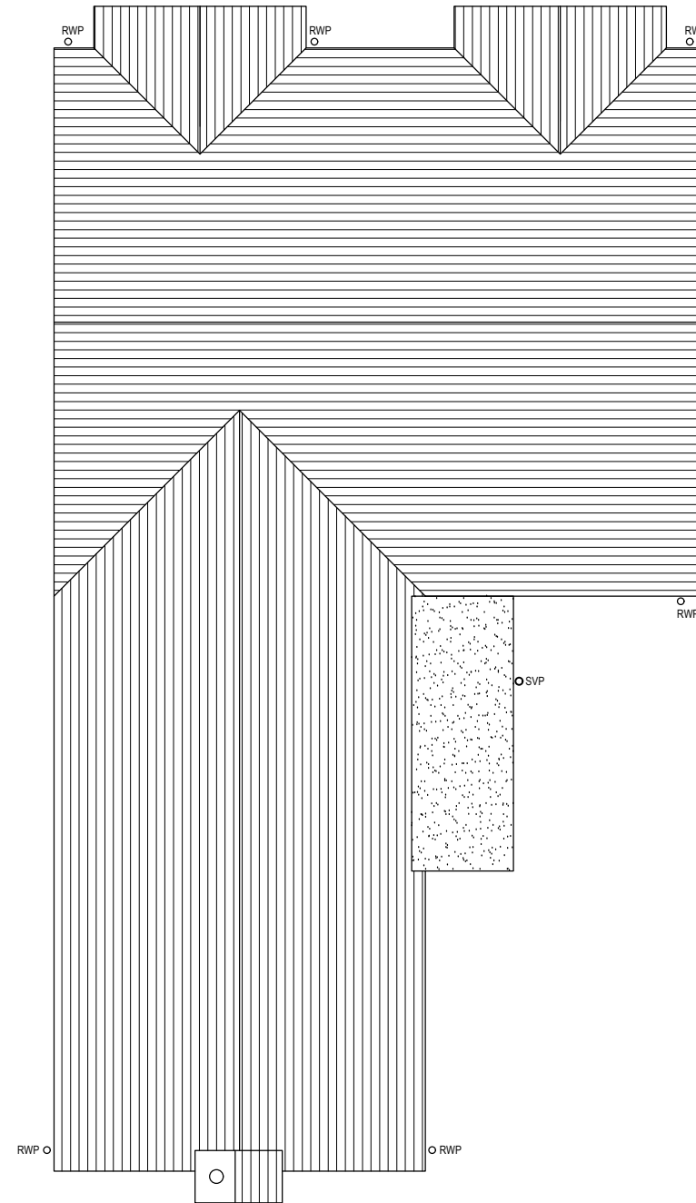
ROOF PLAN
