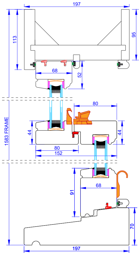
Section B-B Scale 1:4
