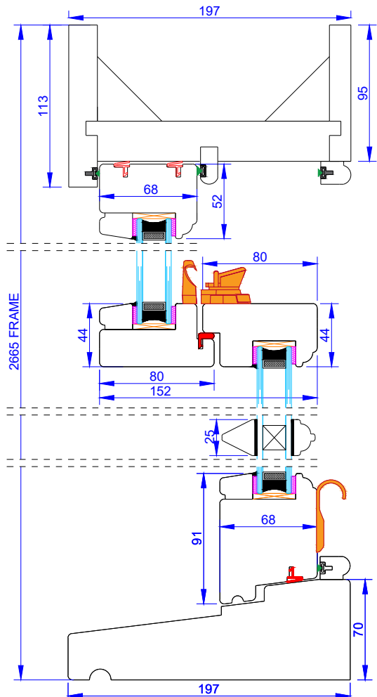
Section B-B Scale 1:4
