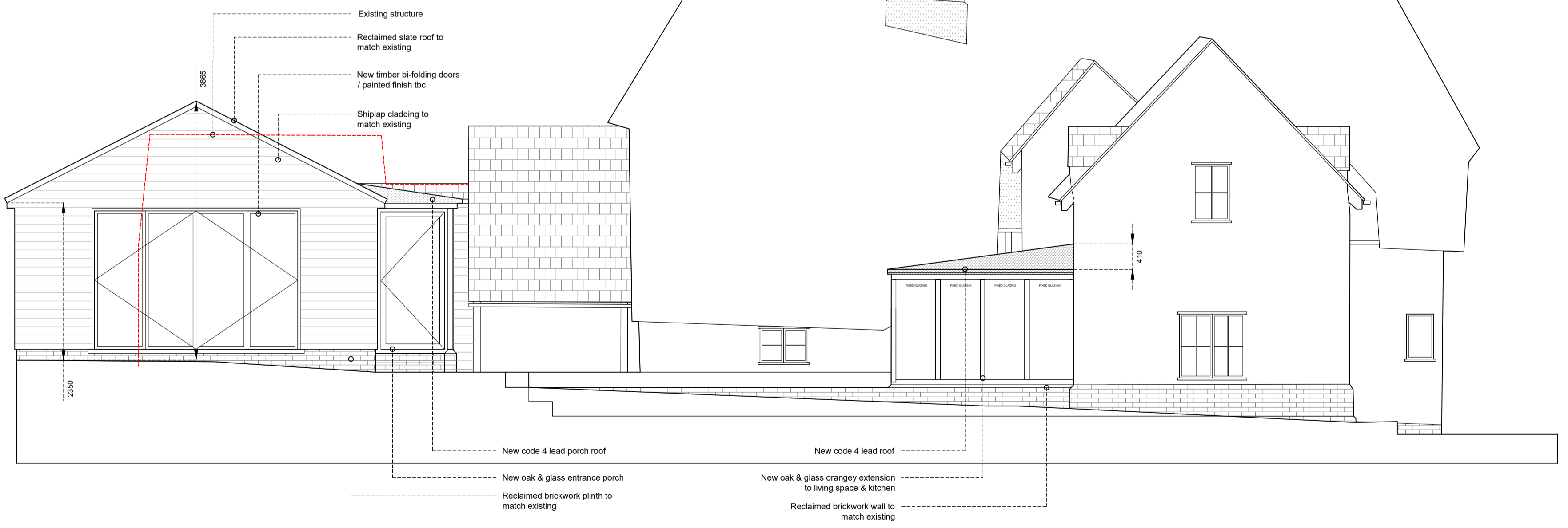
proposed western elevation
