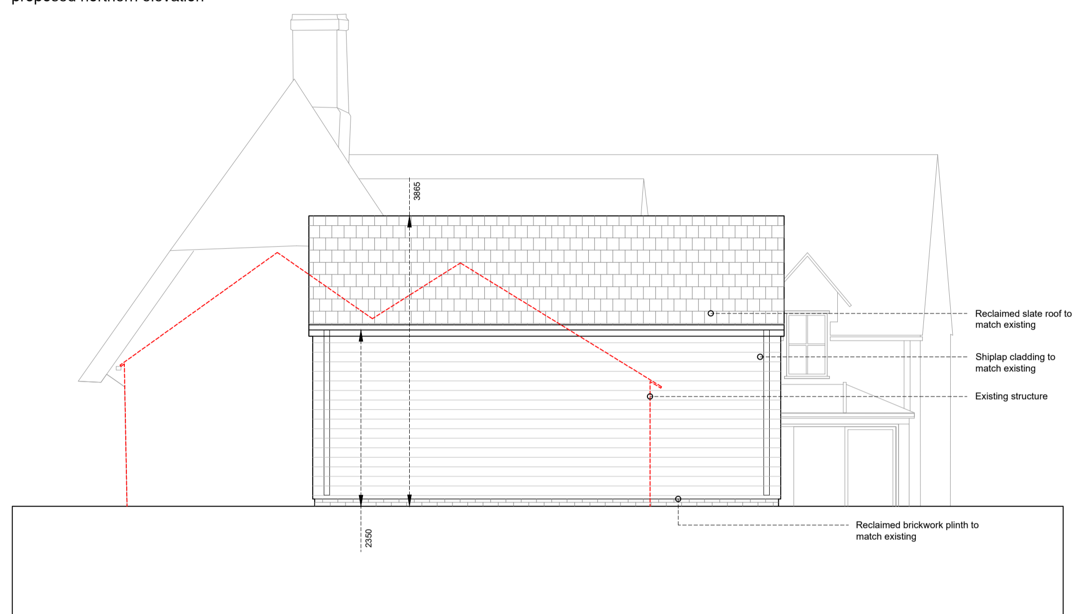
proposed northern elevation
