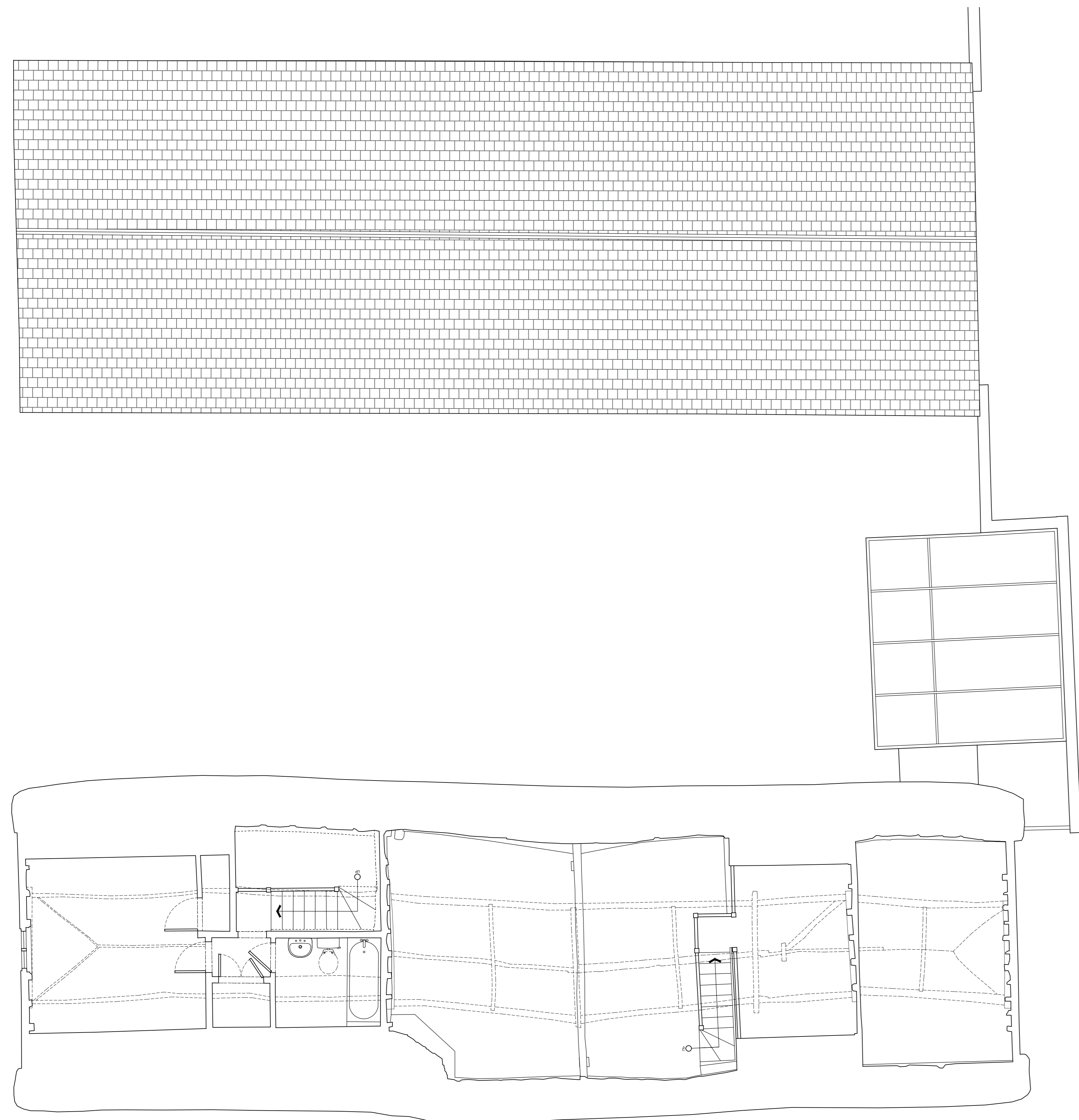
2 1 0.5 0 existing first floor plan
