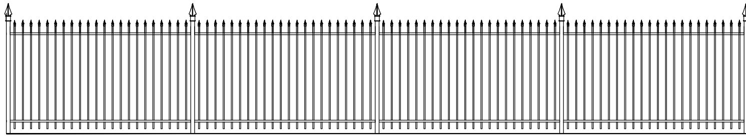
Proposed Fence Elevation scale 1:50@A3
