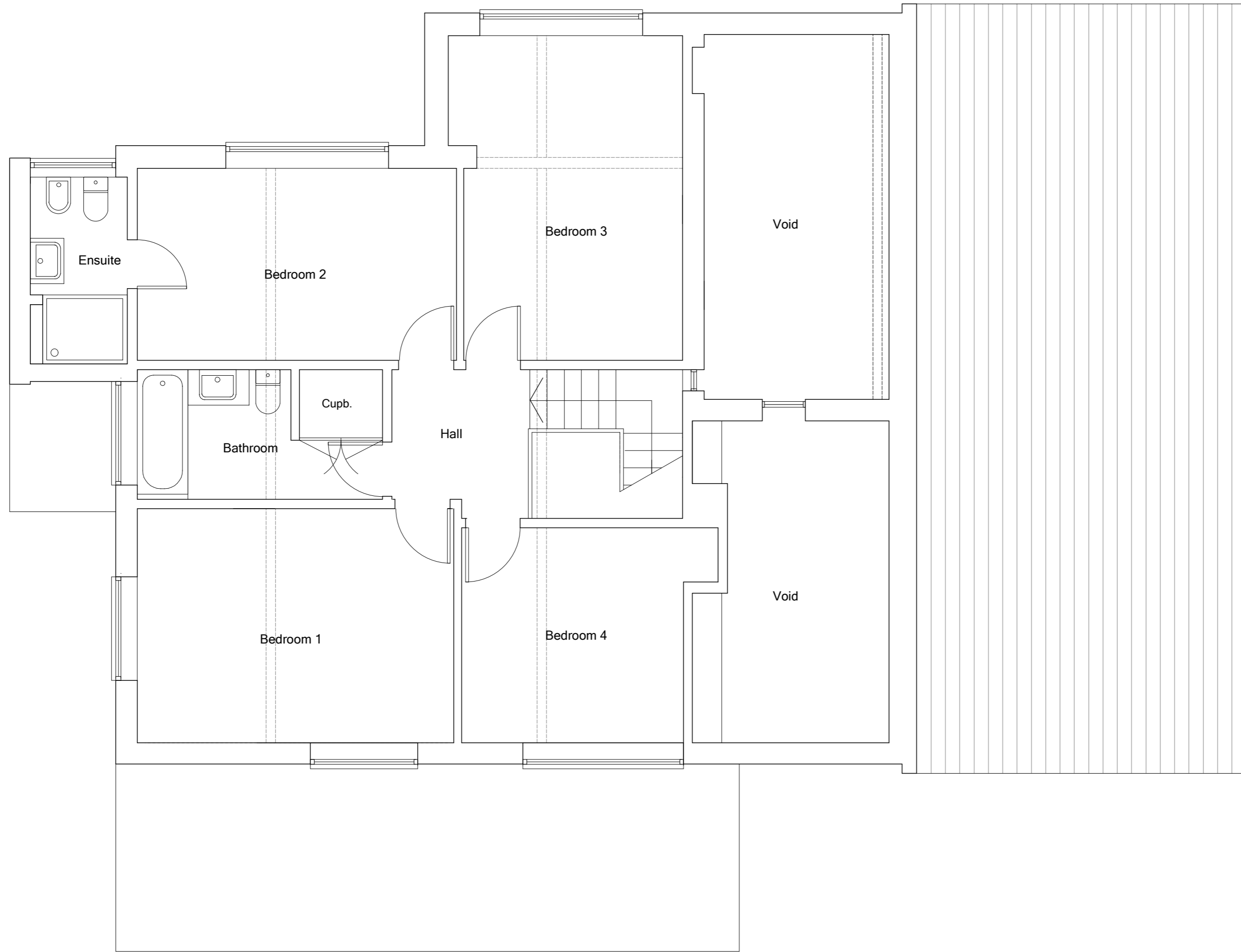
Existing First Floor Plan scale 1:50 @ A2
