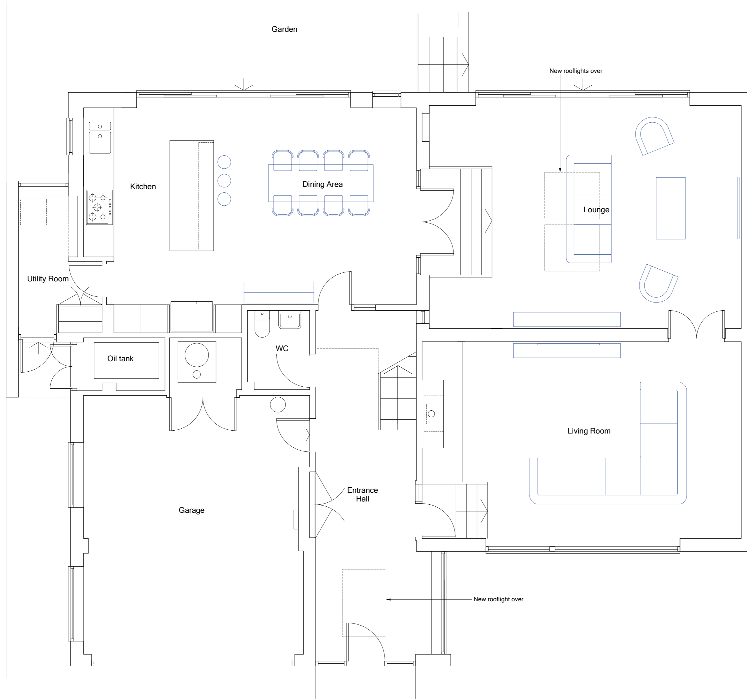
Proposed Ground Floor Plan scale 1:50 @ A2
