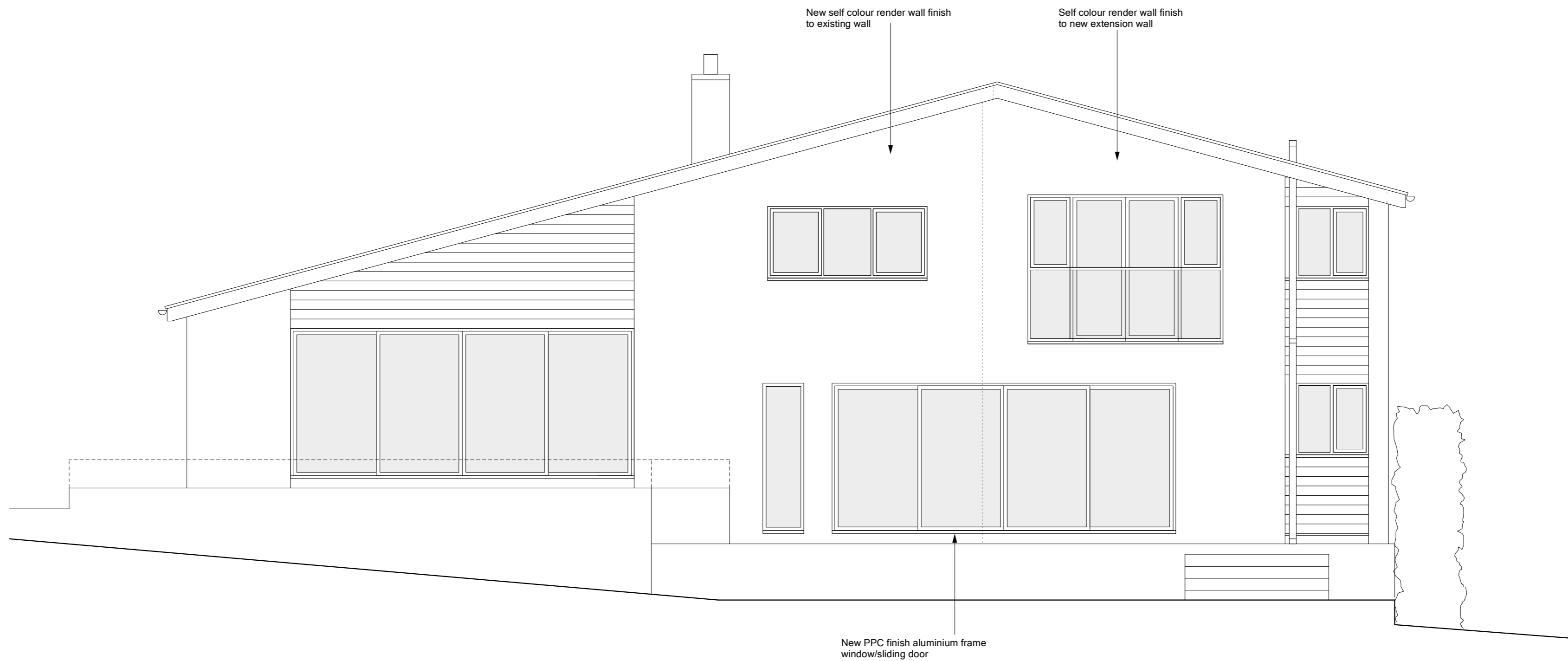
Proposed Rear Elevation scale 1:50 @ A2
