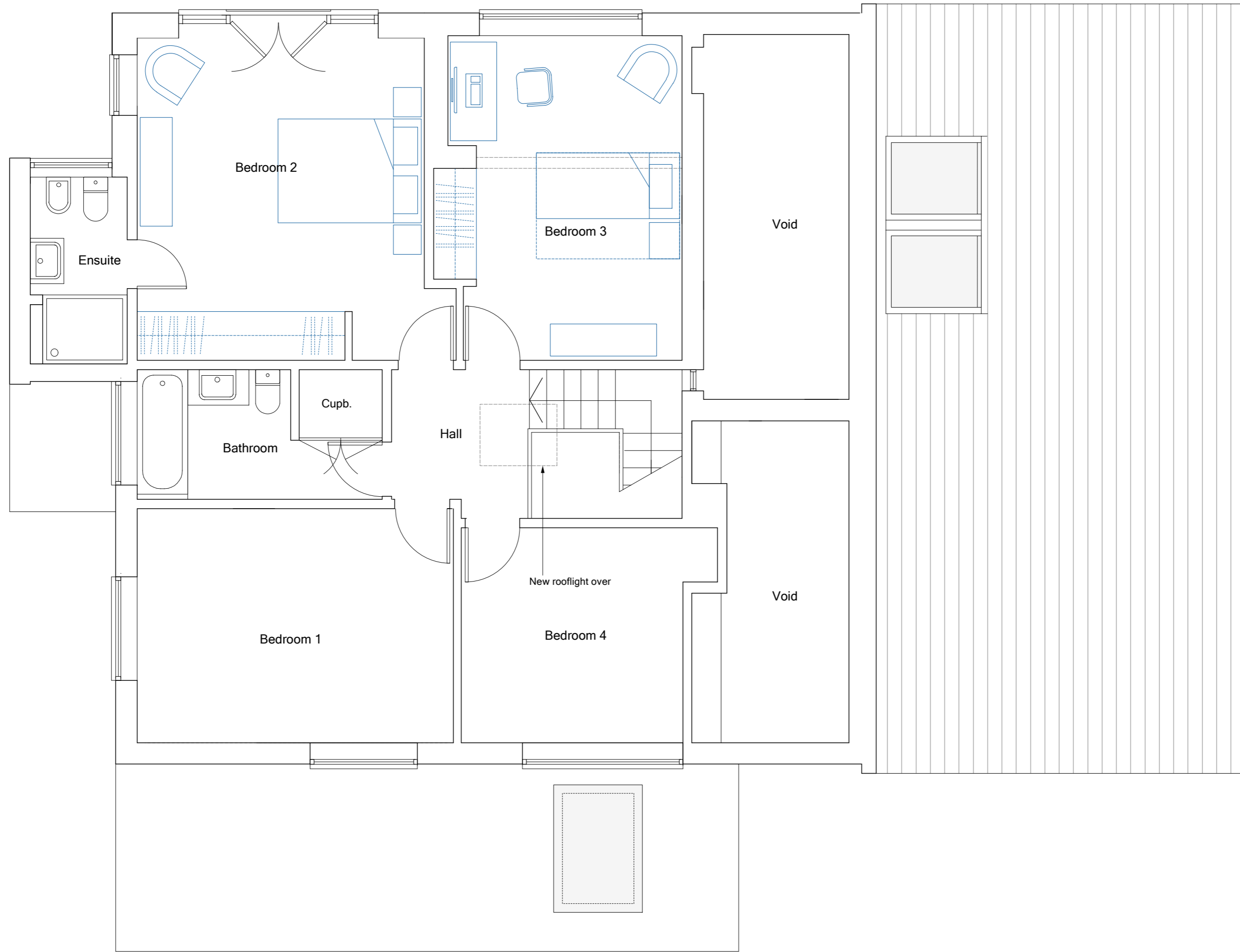
Proposed First Floor Plan scale 1:50 @ A2
