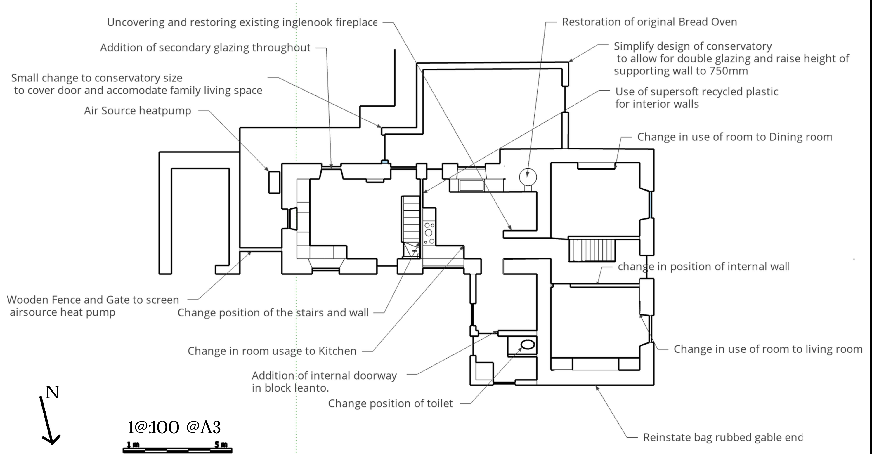
Fig 1. Proposed Ground Floor Plan Polanguy Farmhouse 26/5/23
