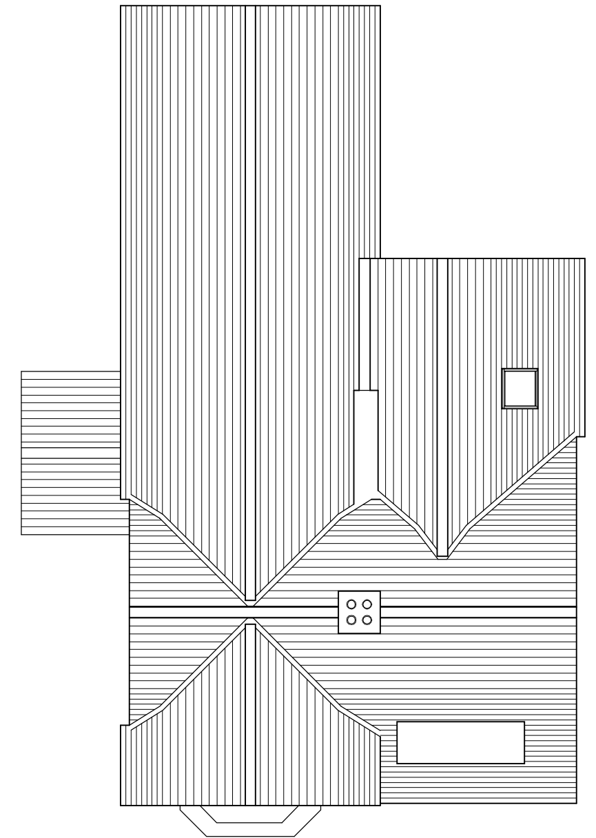
Roofscape Layout
