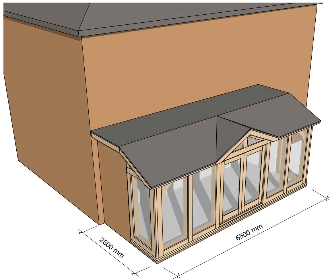
PERSPECTIVE VIEW WITH ROOF REMOVED Scale N/A
