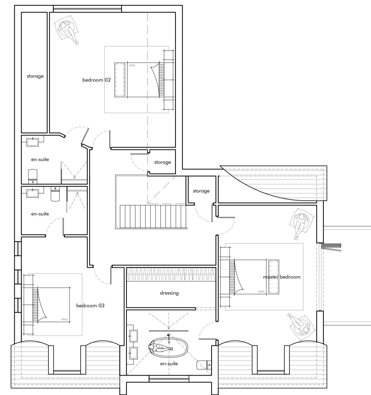
existing first floor plan 146 sqm / 1,571 sqft
