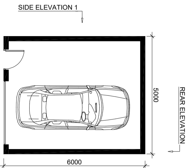
GARAGE PLAN AS EXISTING
