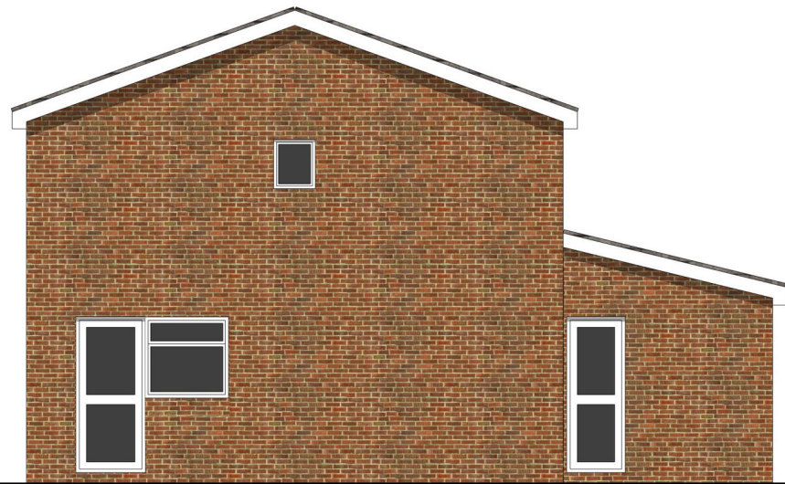
existing side elevation 1 scale 1:100
