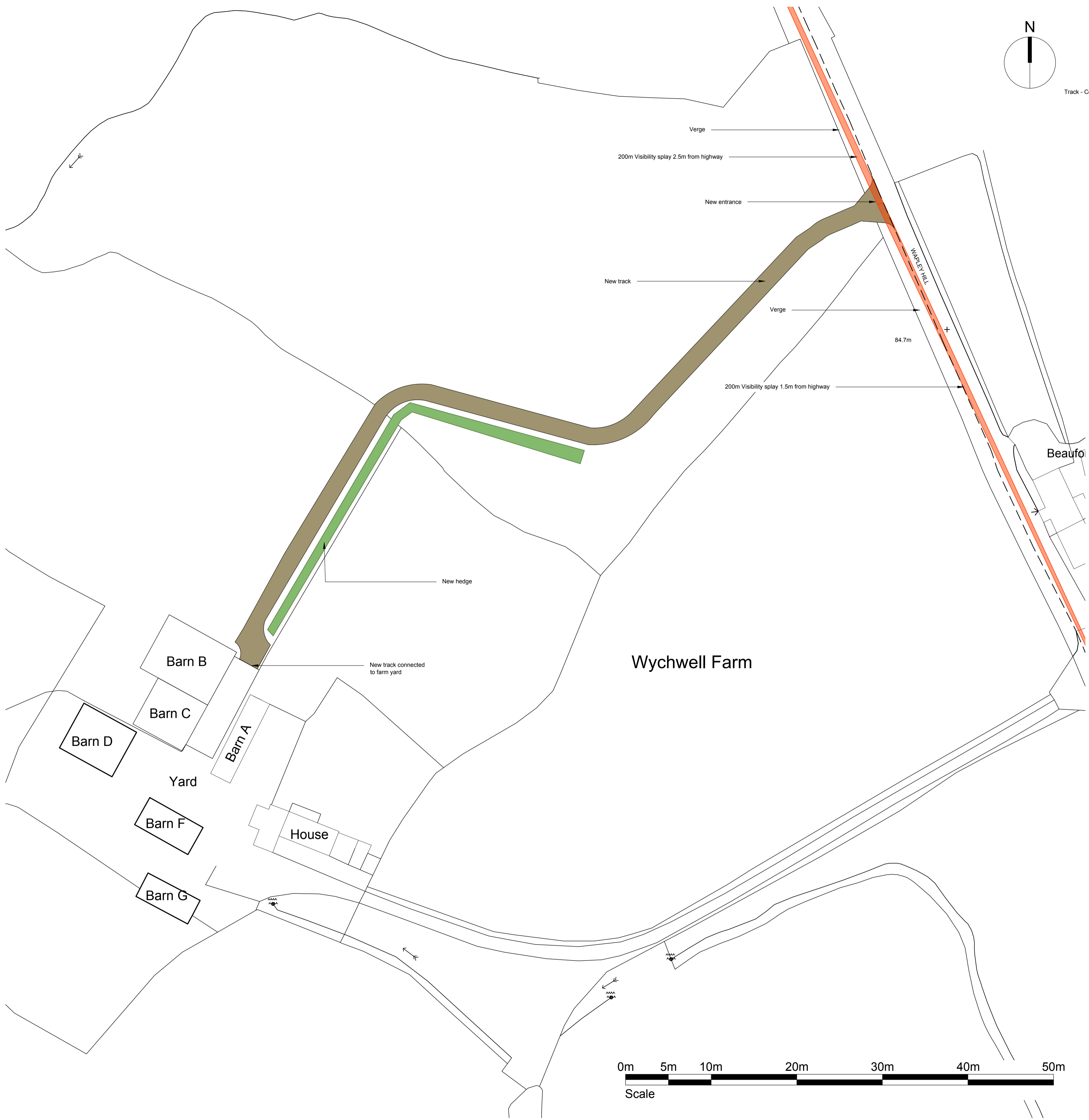
Proposed Site Plan Scale: 1:500
