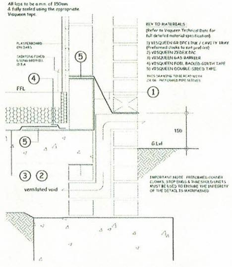
Typical Suspended Slab - Option B (GB-12)
