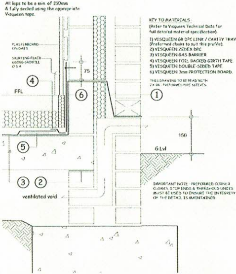
Typical Suspended Slab - Option A (GB-10)
