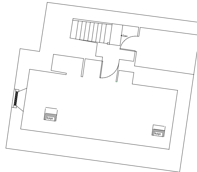
Proposed Second Floor 1:100
