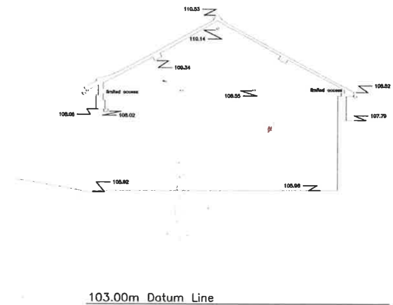
SECTION E
