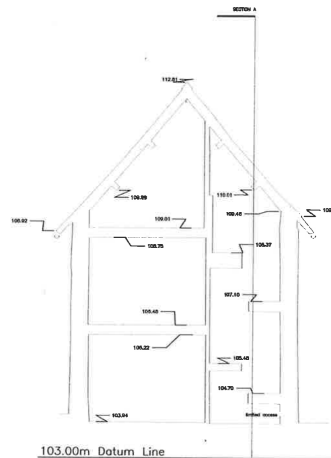
SECTION D
