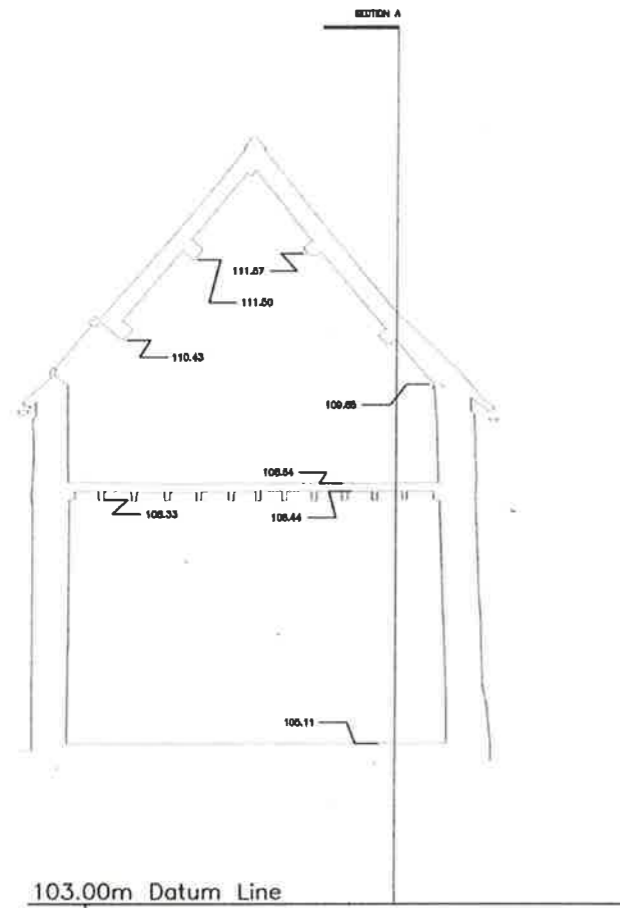
SECTION C
