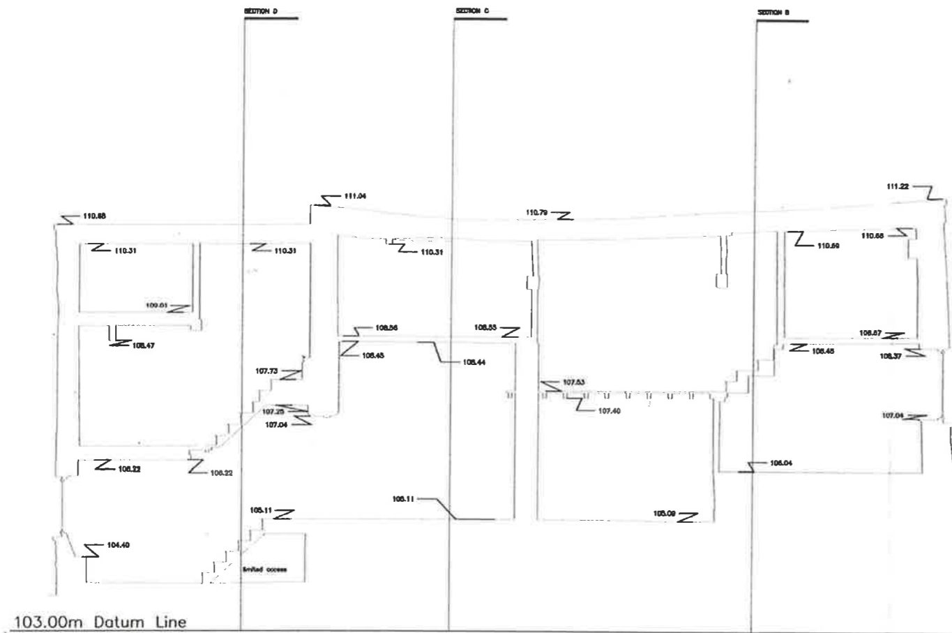
SECTION A
