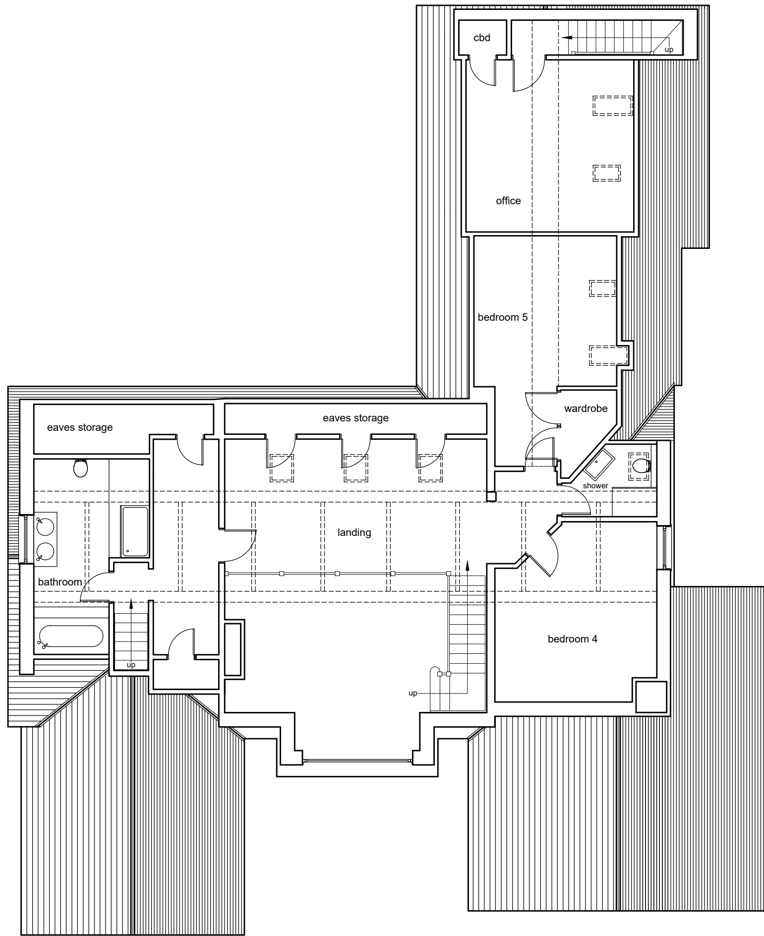
first floor plan as existing 1:100
