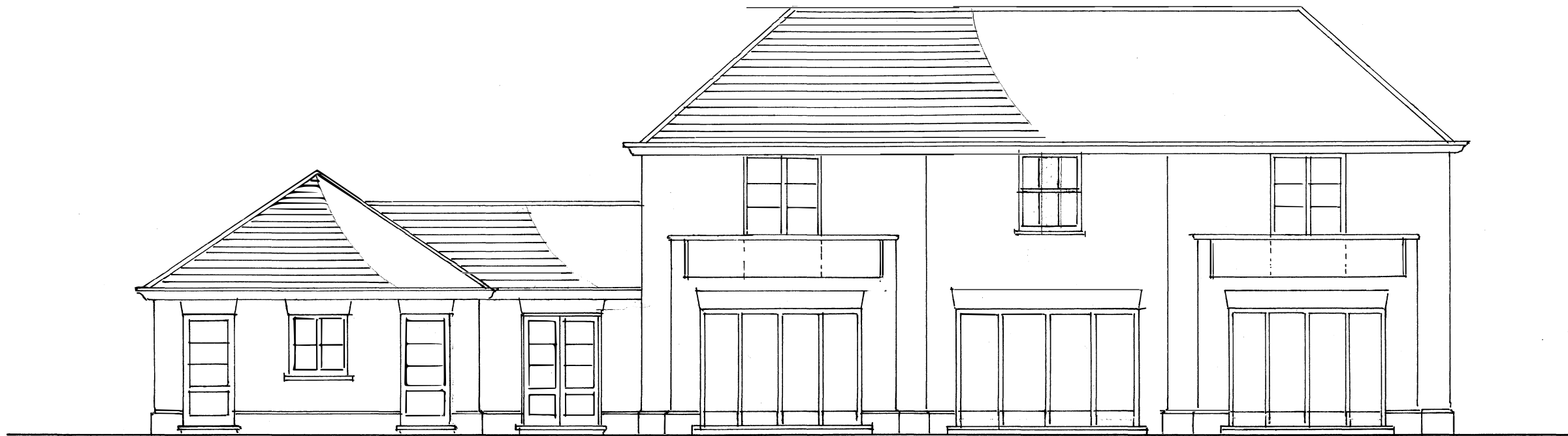
NORTH GARDEN ELEVATION
