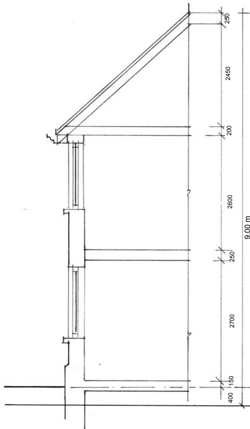
PART SECTION FRONT WALL
