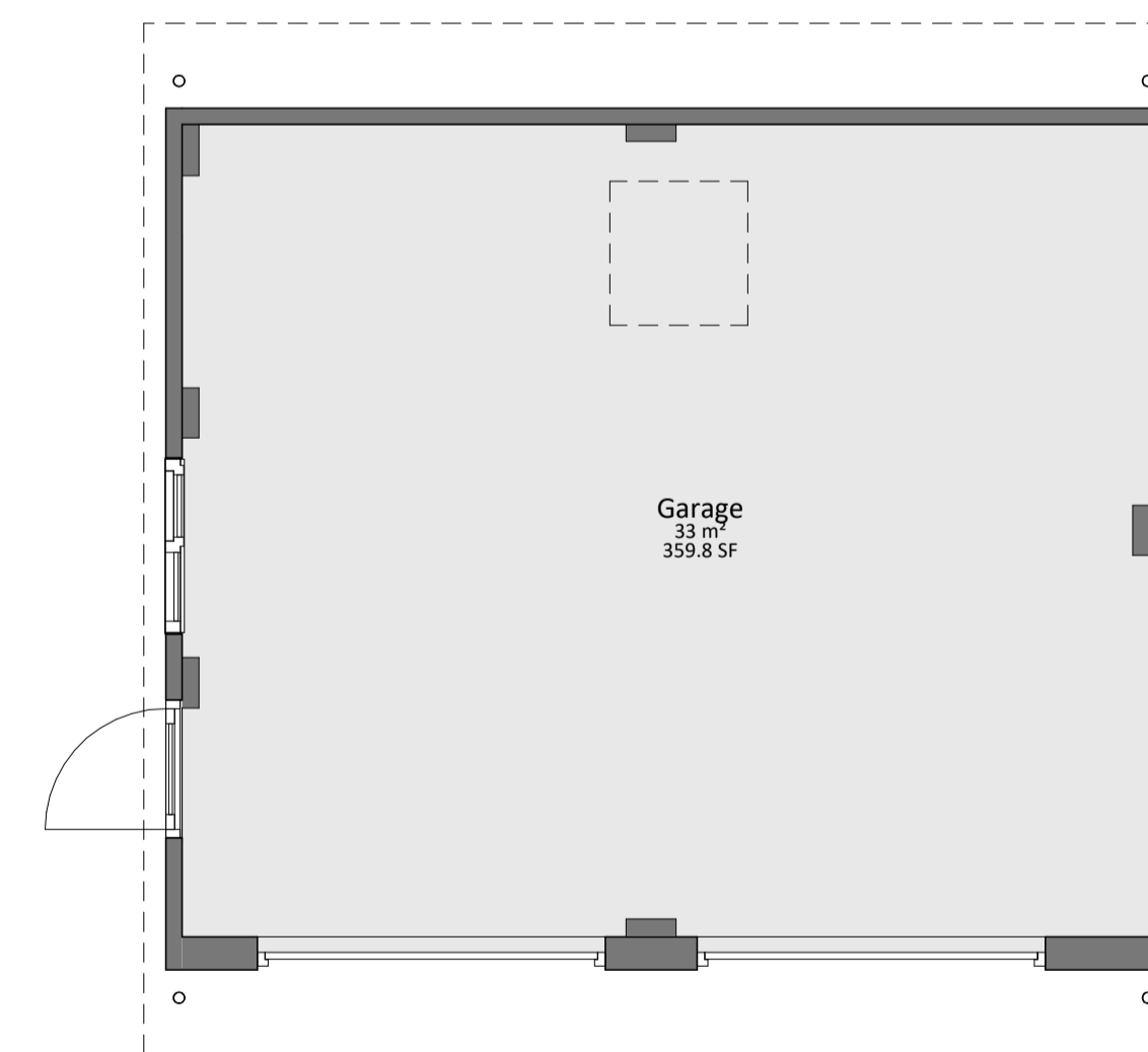
Existing 00 Plan 1 : 50
