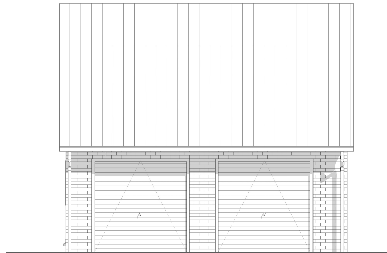
South Elevation 1 : 50
