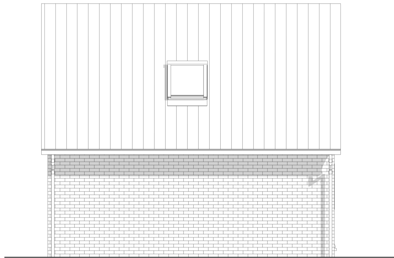
North Elevation 1 : 50
