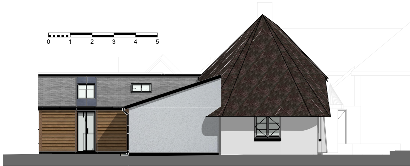
1 Elevation South West (Proposed) 1:100
