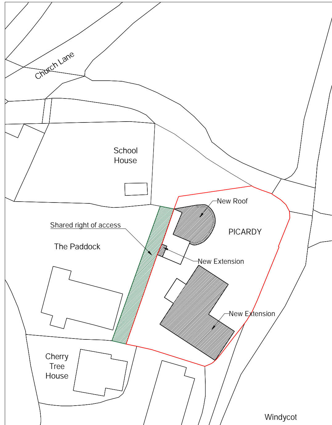
Proposed - SITE PLAN (BLOCK PLAN) 1:500
