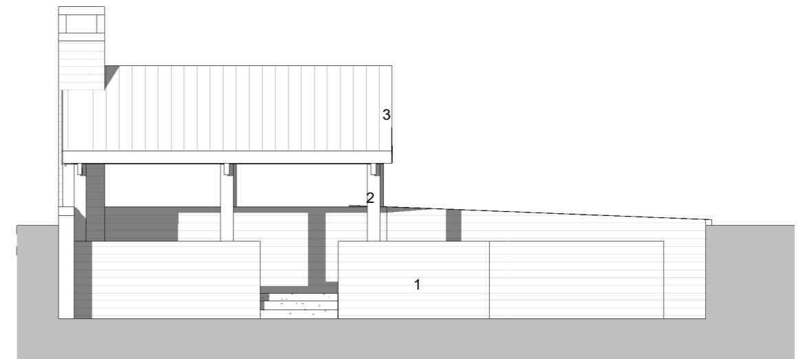
Front Elevation 1 : 100
