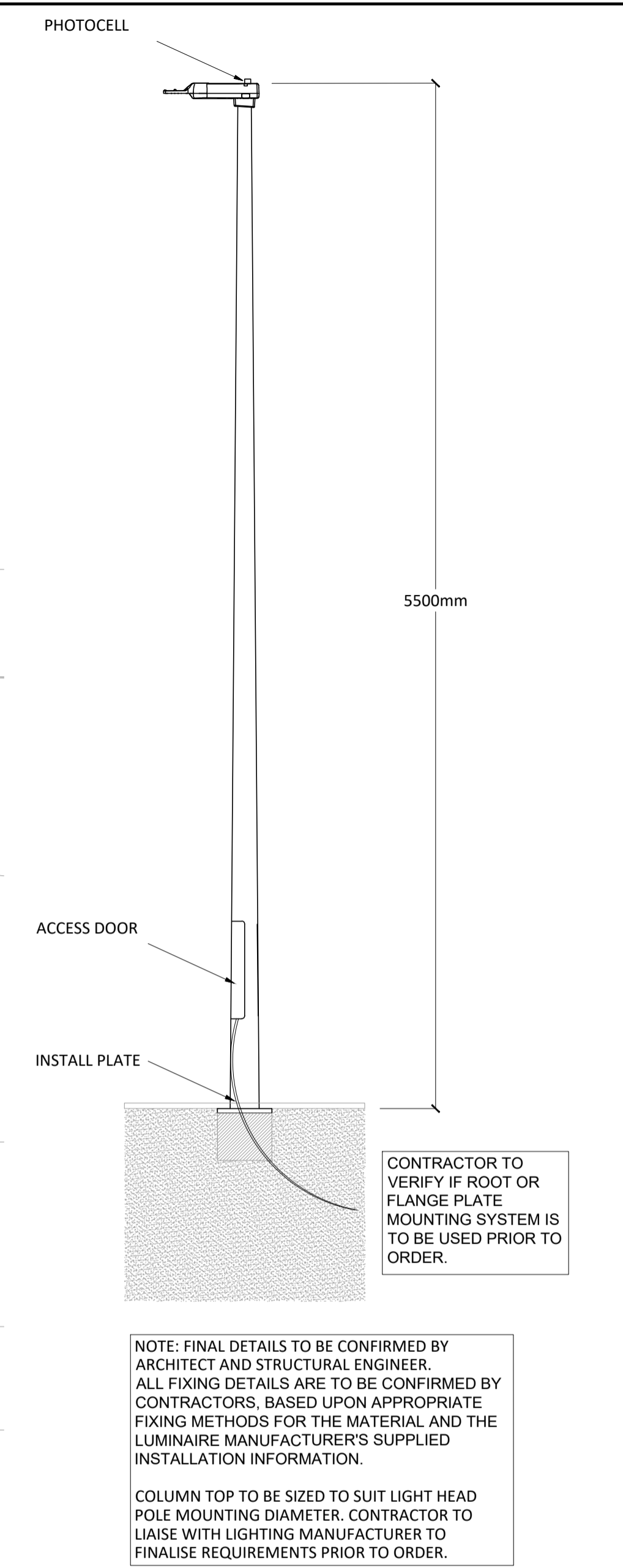
COLUMN DETAIL SCALE 1:25@A1
