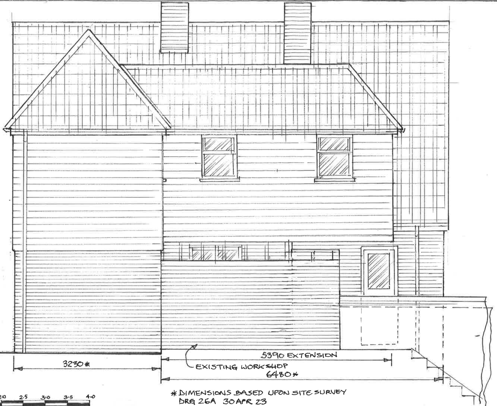
18 D PROPOSED BATHROOM EXTENSION SIDE VIEW 1:50
