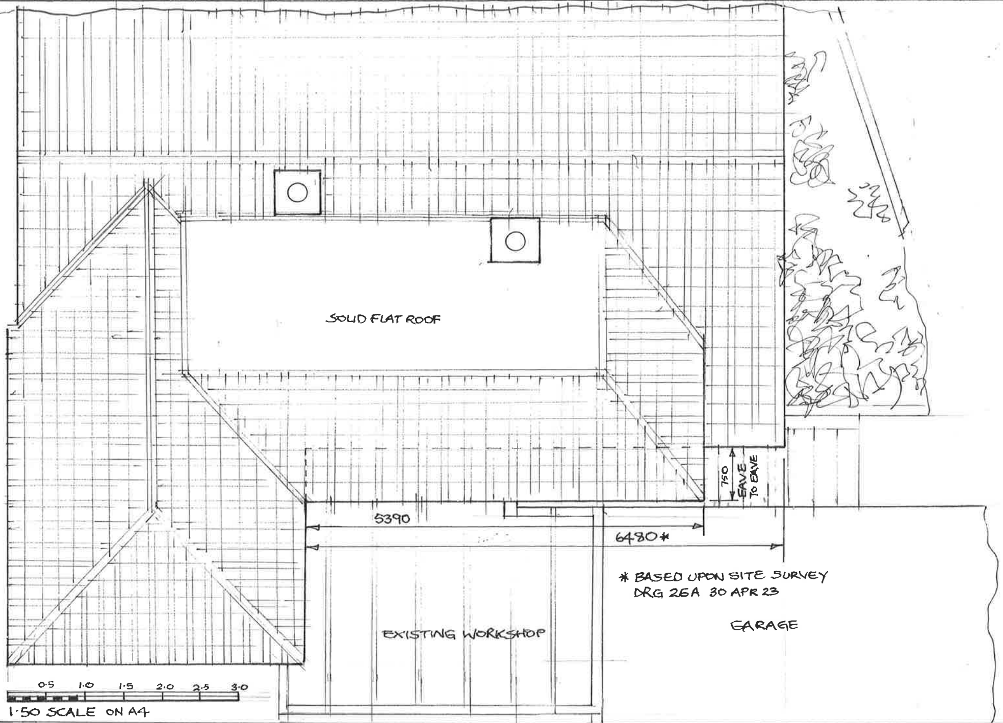
19 E PROPOSED BATHROOM EXTENSION ROOF PLAN 1:50
