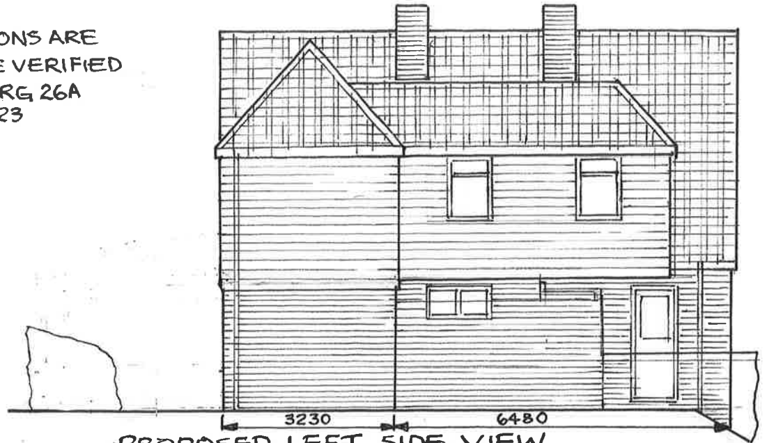
PROPOSED LEFT SIDE VIEW ABOVE WORKSHOP + GARAGE
