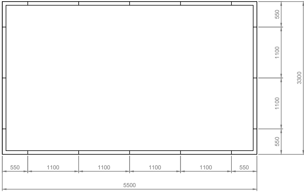
PLAN SECTION
