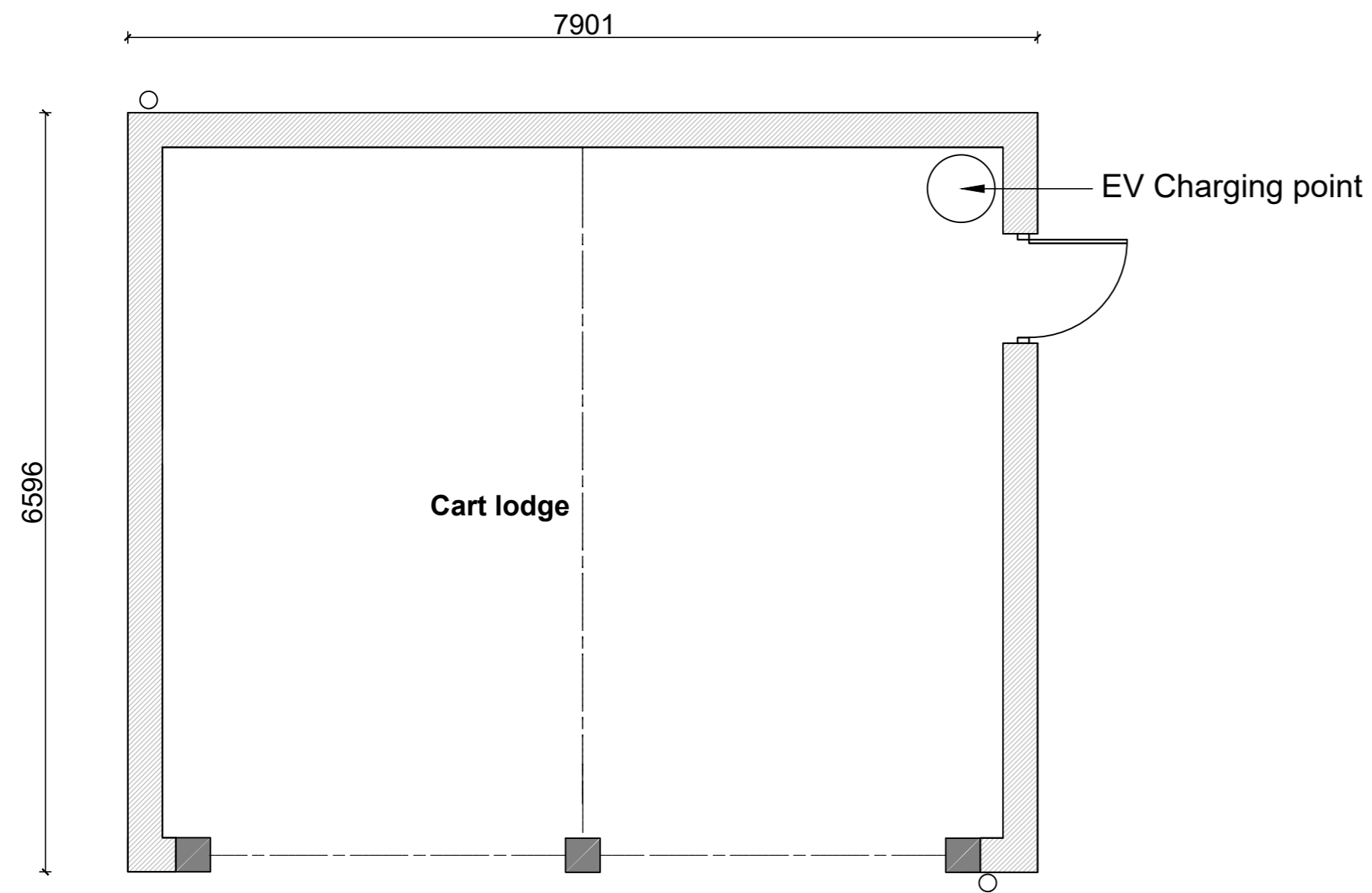
Cartlodge Floor Plan
